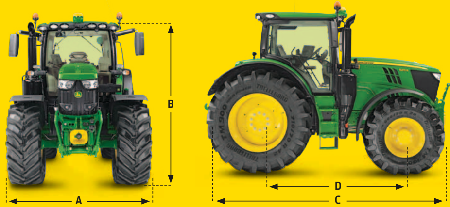
(A) Width: 2550 mm (B) Total height: 3160 mm (C) Overall length: 5050 mm (D) Wheelbase: 2800 mm
